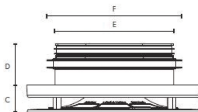
Side view [Based on drawing of RV 125]
